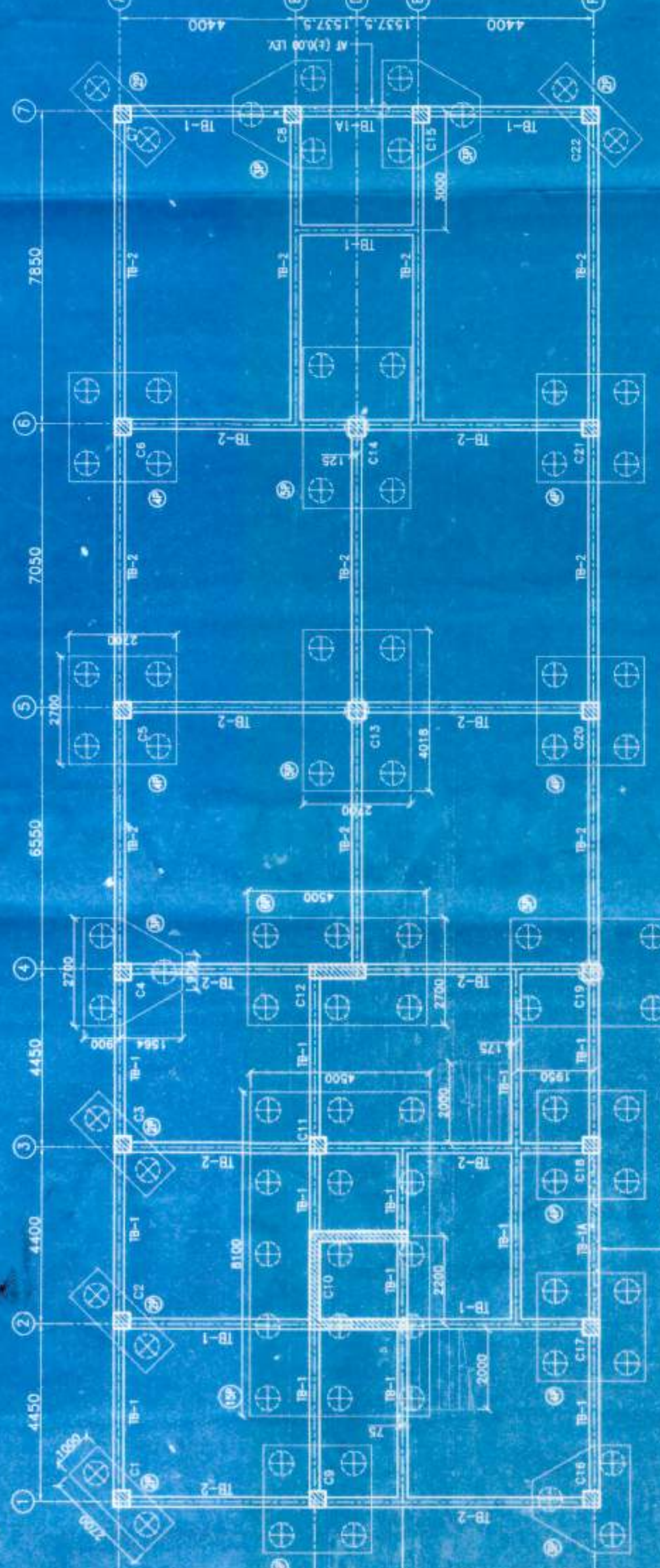
FOUNDATION & TIE BEAM LAYOUT
