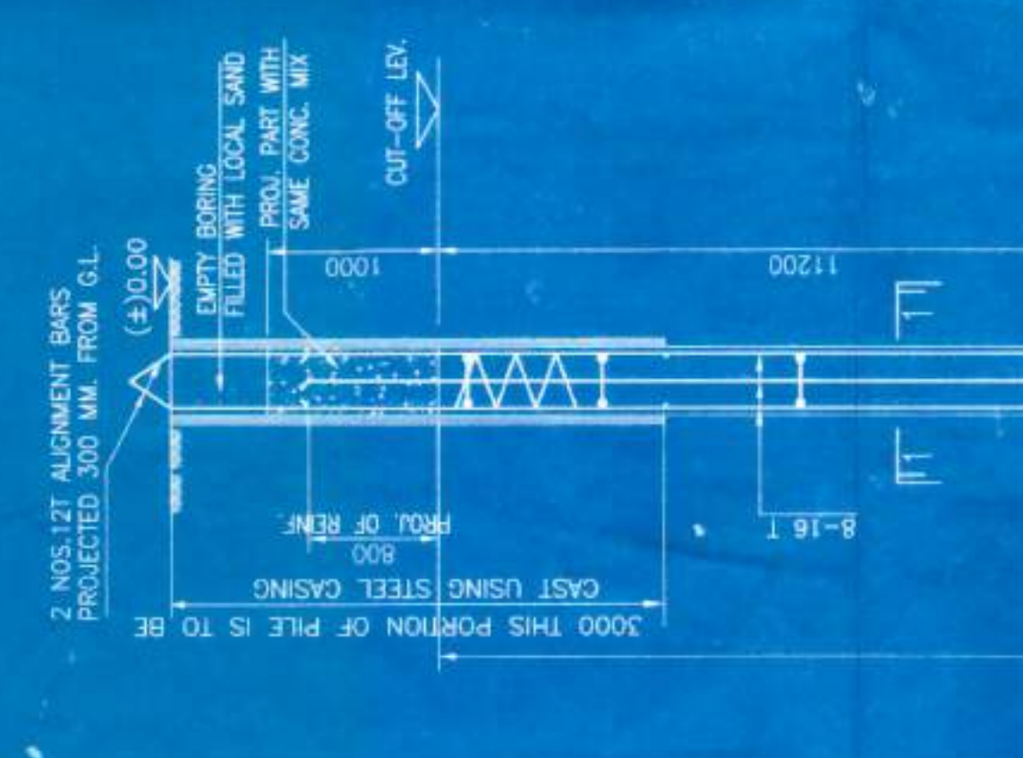
SECTION 1-1
