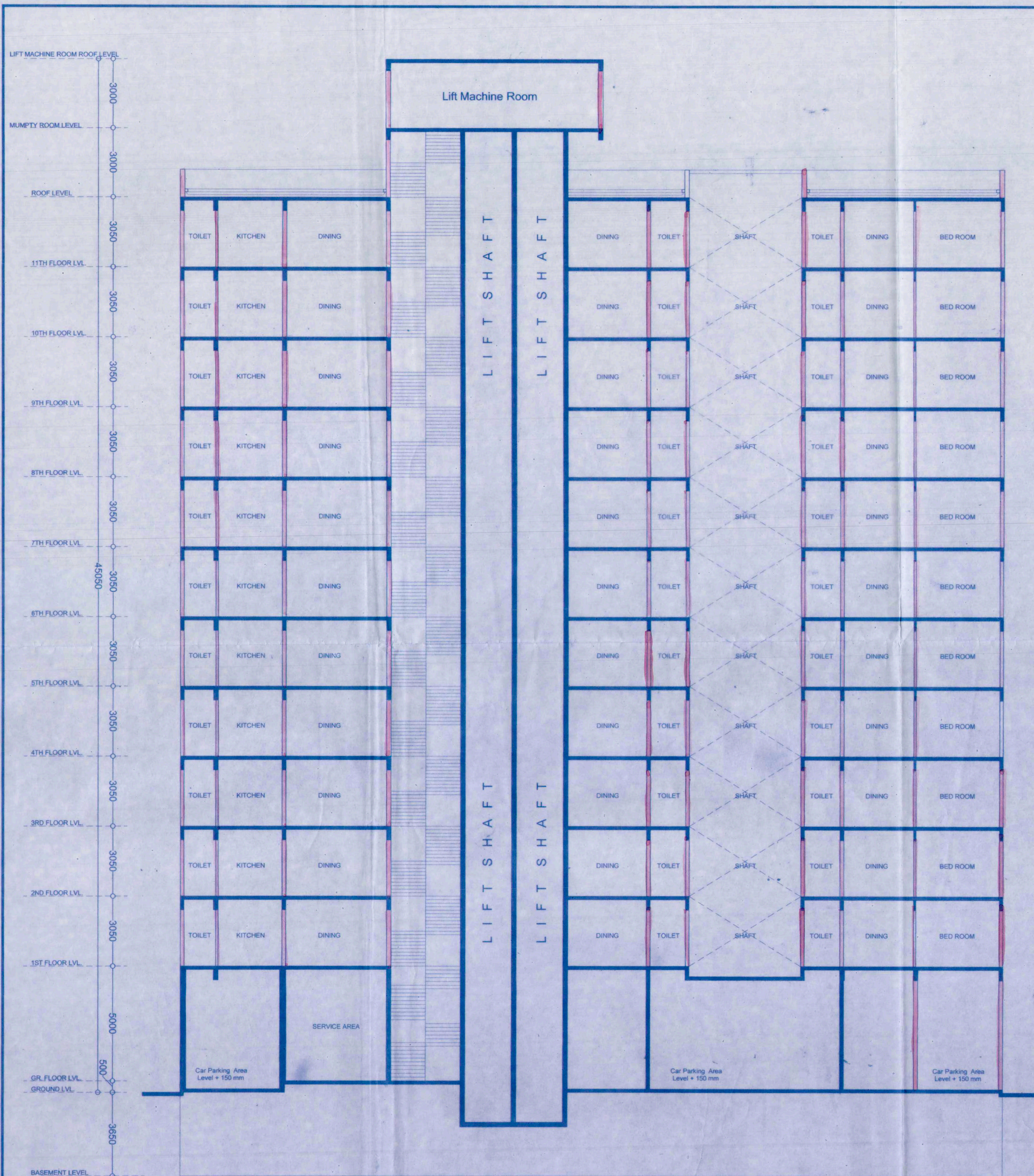
SECTION-EE SCALE-1:100
