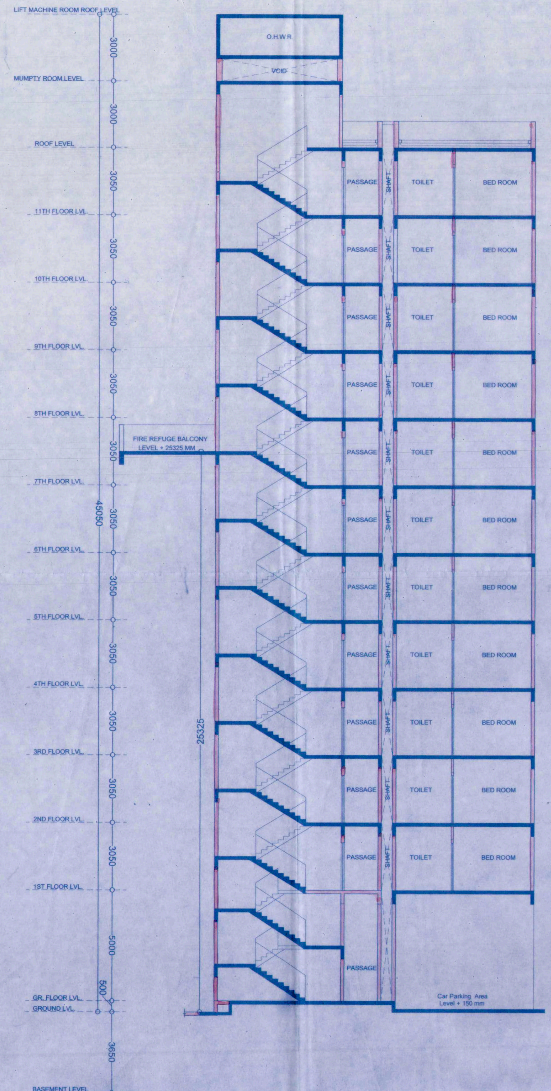
SECTION-FF SCALE-1:100
