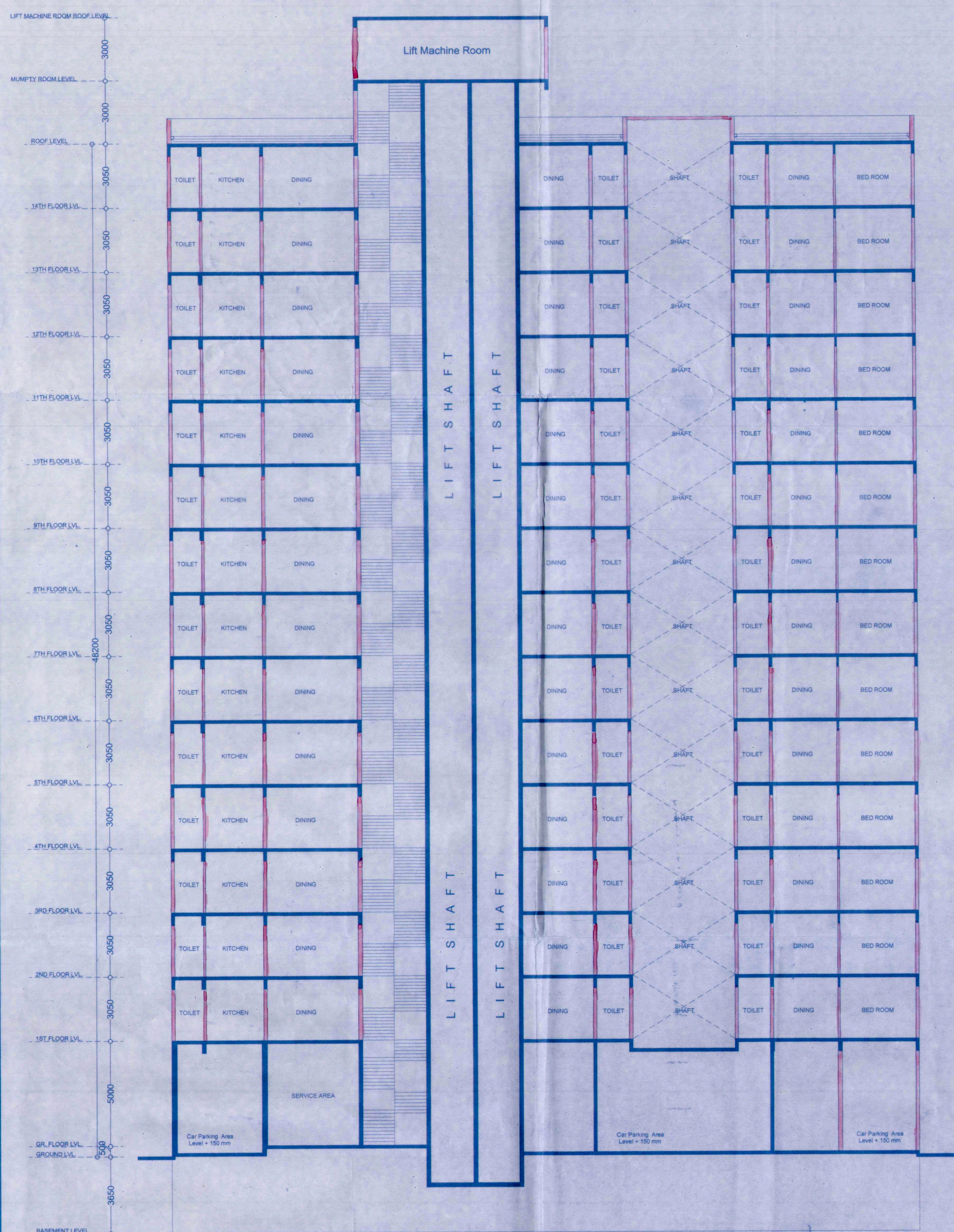
SECTION-CC SCALE-1:100
