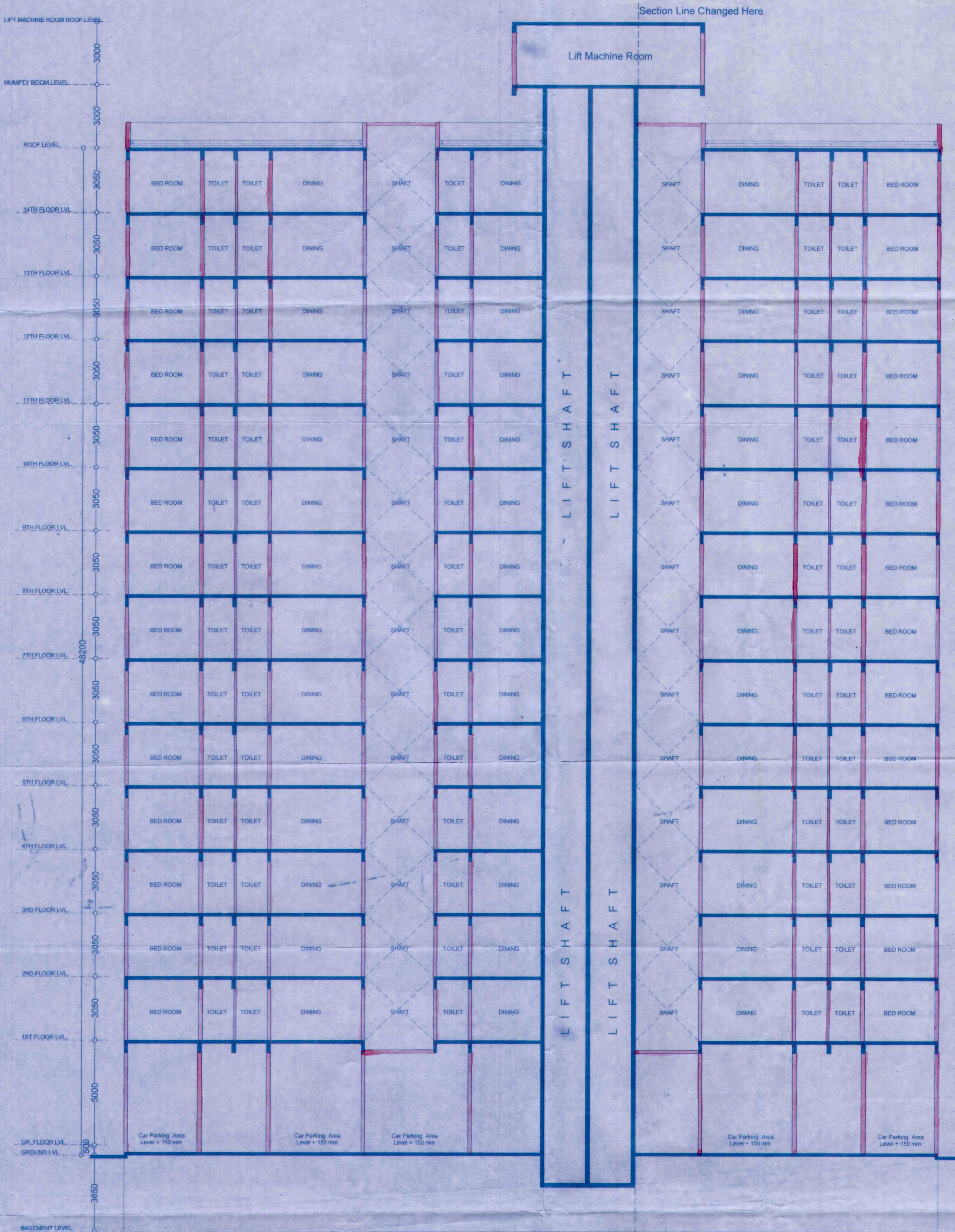
SECTION-AA SCALE-1:100
