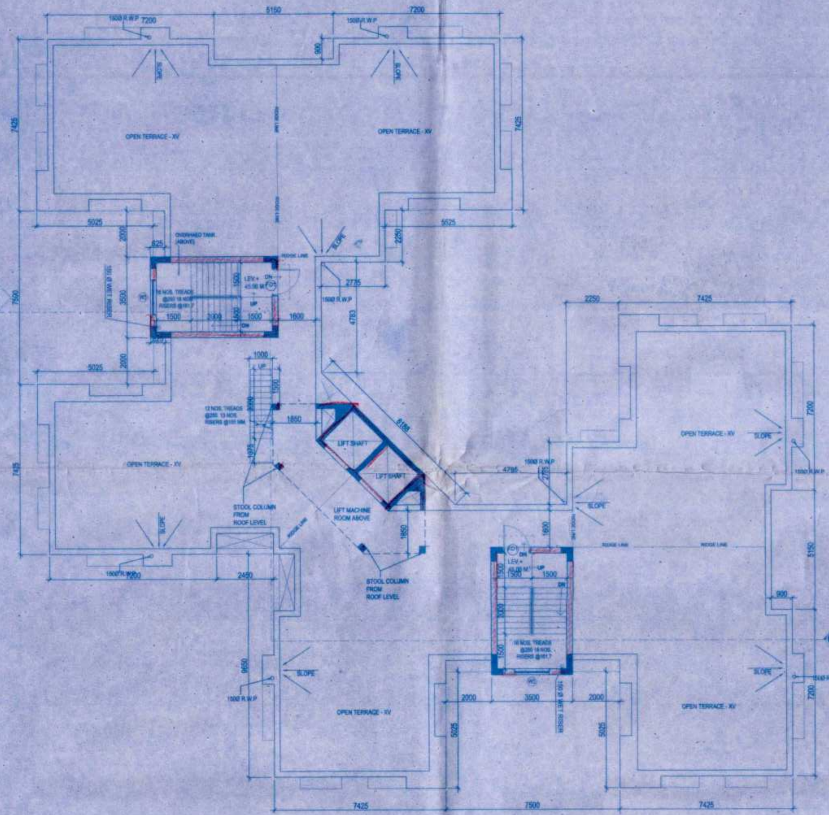
ROOF PLAN
