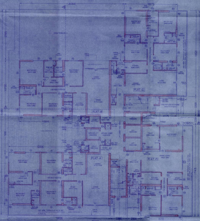
35TH FLOOR PLAN SCALE-1:100
