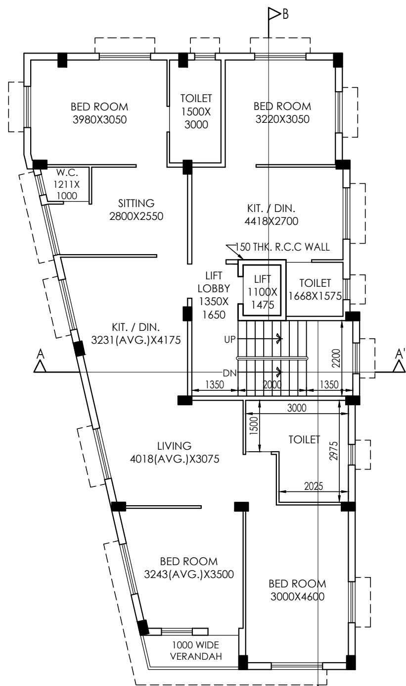
1ST FLOOR PLAN SCALE - 1:100
