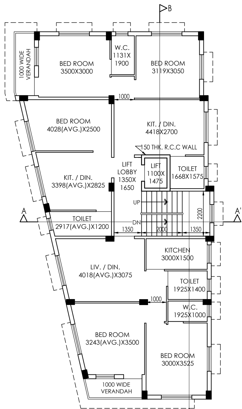
2ND & 3RD FLOOR PLAN SCALE - 1:100
