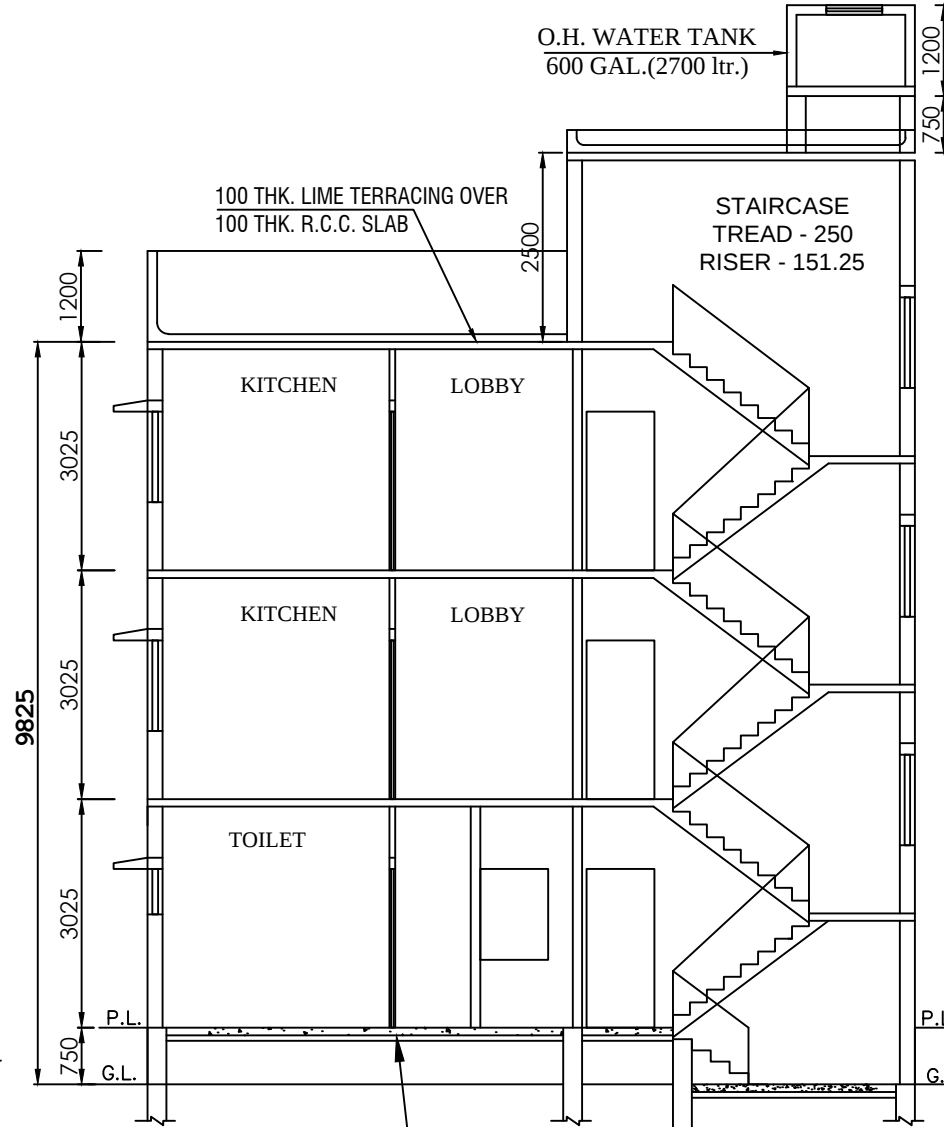
SECTION - "B-B"
