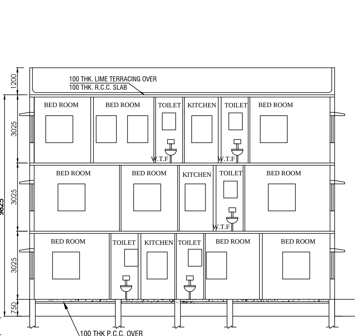
SECTION - "A-A"
