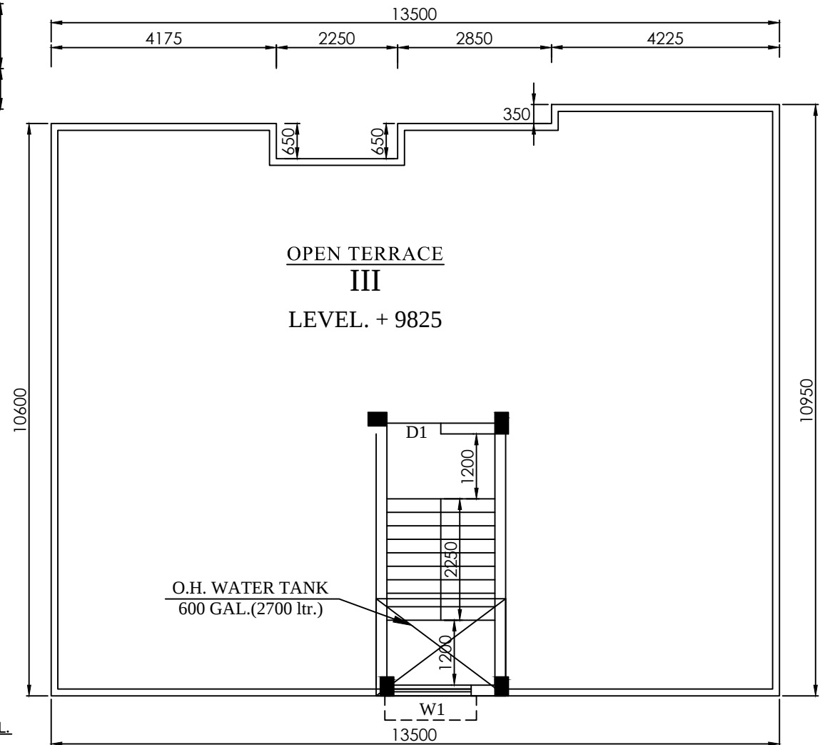
ROOF PLAN
