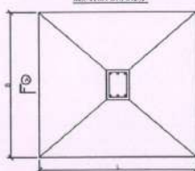
DETAILS OF ISOLATED FOUNDATION SCALE: 1:20
