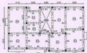
BEAM & SLAB LAYOUT PLAN SCALE: 1:100
