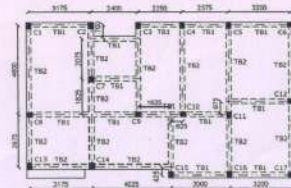
TIE BEAM LAYOUT PLAN SCALE: 1:100
