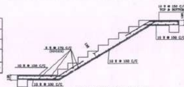
DETAILS OF STAIR SLAB SCALE: 1:20
