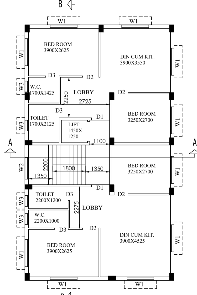
SECOND & THIRD FLOOR PLAN
