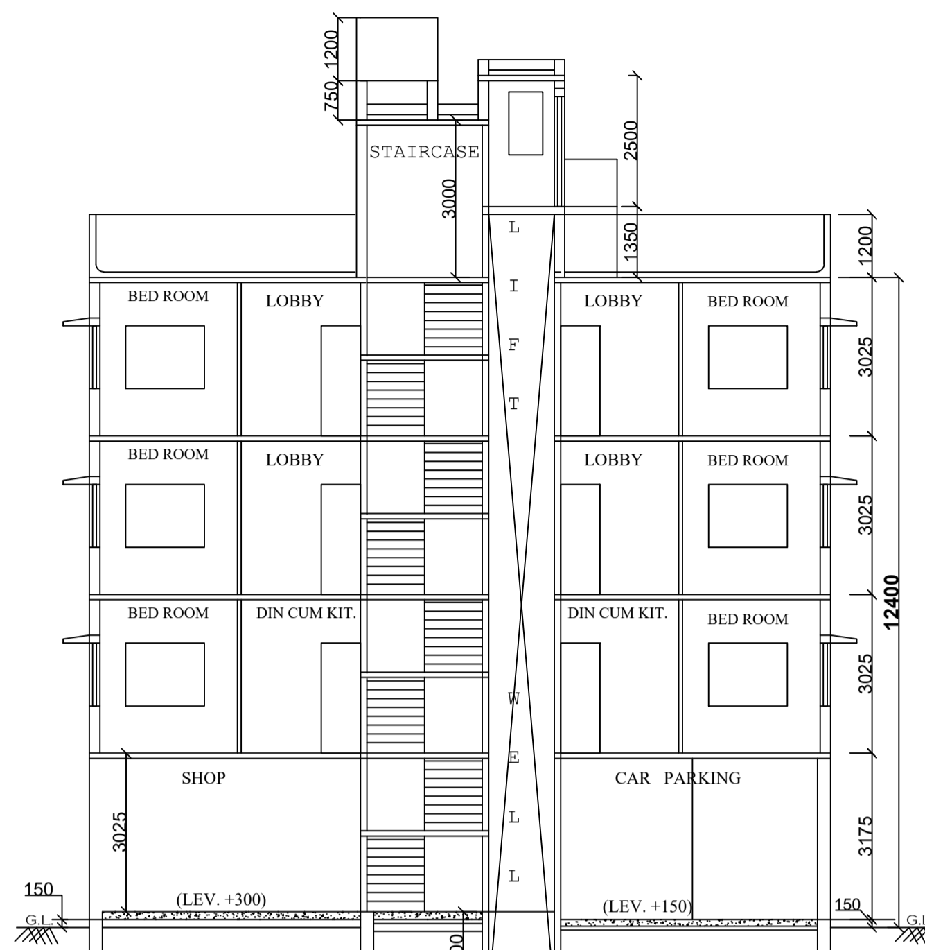
SECTION - "B-B"
