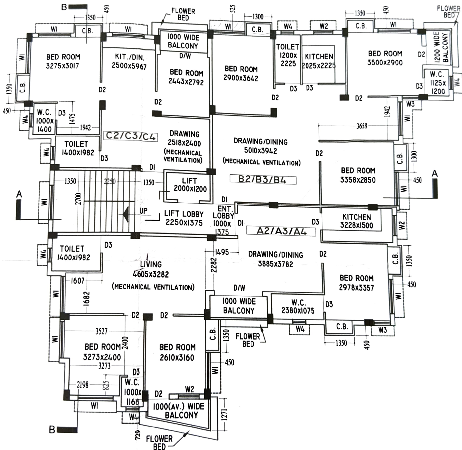
2ND, 3RD, 4TH FLOOR PLAN
