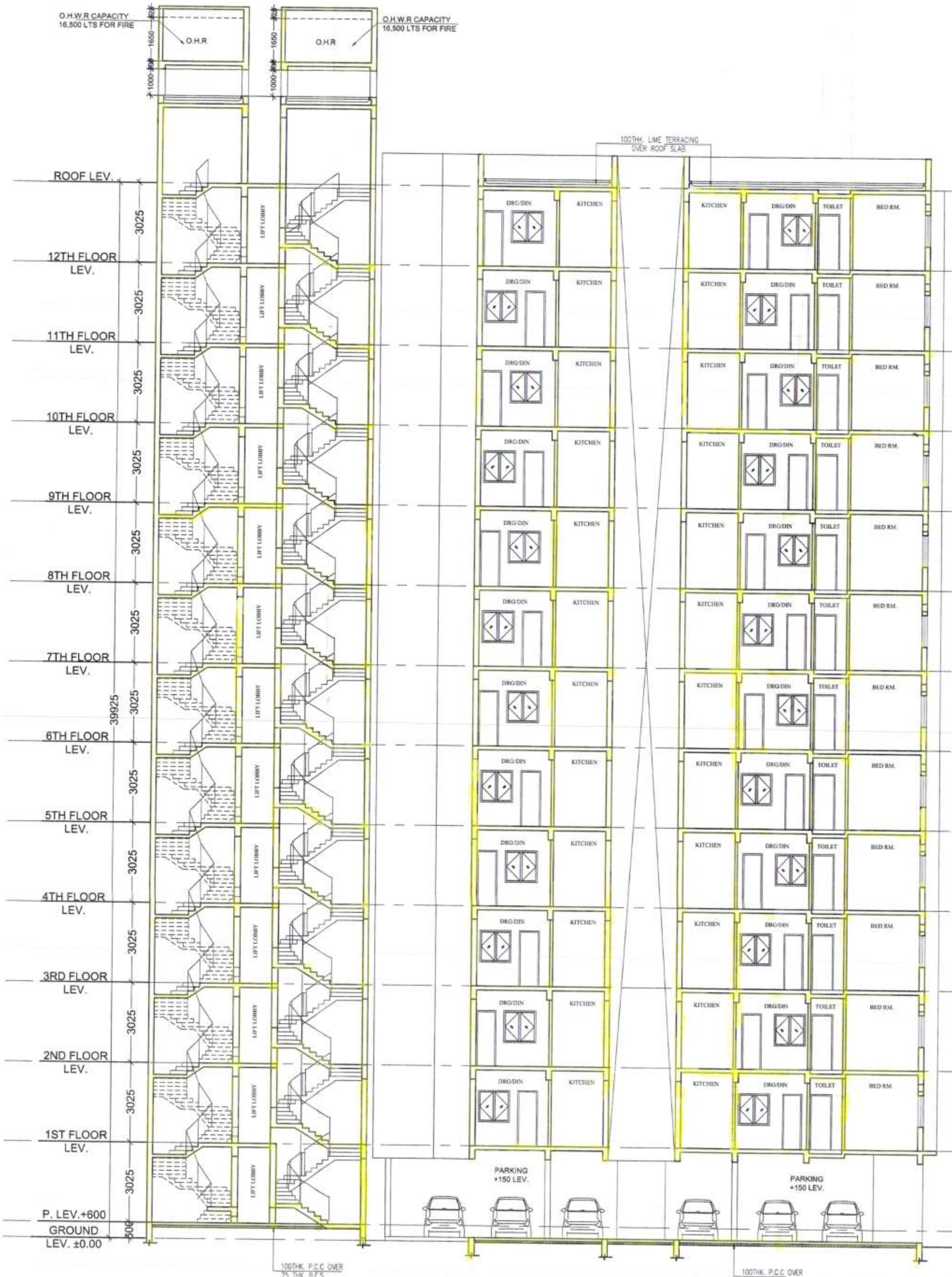
SECTION - B-B
