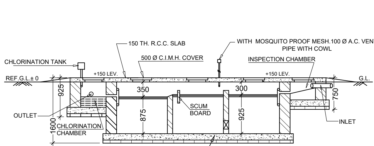
SECTION = M - M
