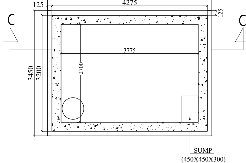
DETAIL OF S. U.G.W. RESERVOIR CAP. : 10,000 LTR. (SCALE -1:50)
