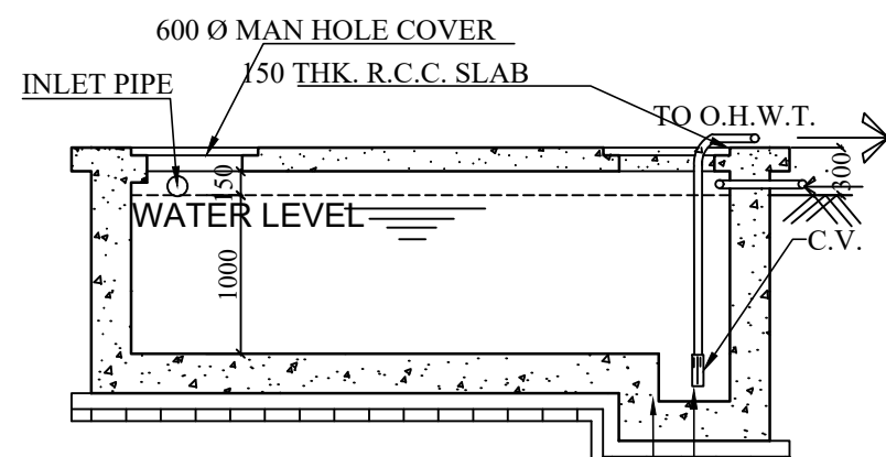
SECTION-C-C
