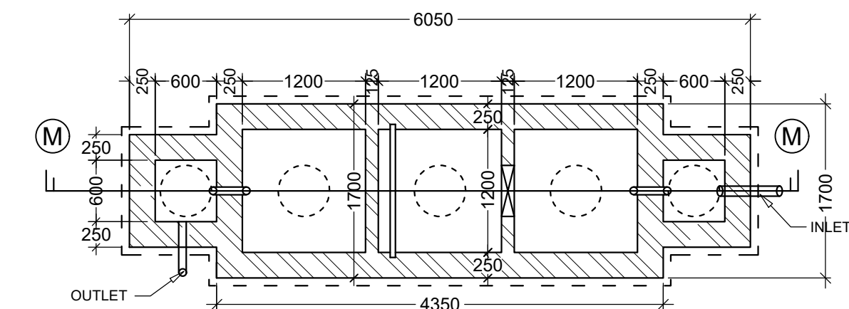
DETAILS OF SEPTIC TANK. (50 USERS) (SCALE- 1:50)
